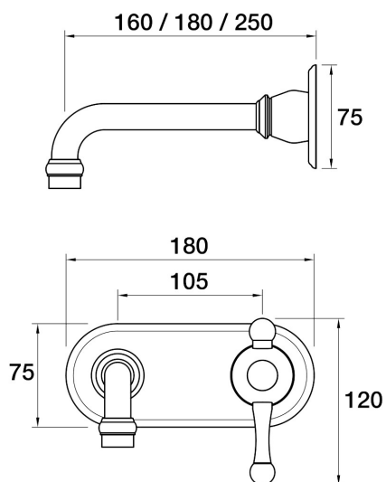
Tudor Wall Bath Mixer Set 160mm outlet Incl. plate A31.041.1.11 - 23k Gold
