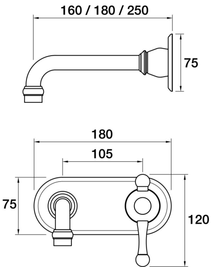
Tudor Wall Bath Mixer Set On Plate 250mm A31.041.4.01 - Chrome
