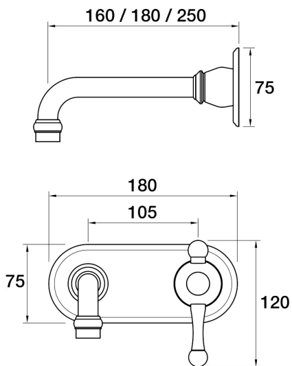
Tudor Wall Bath Mixer Set 250mm outlet Incl. plate A31.041.4.41 - Brushed Brass
