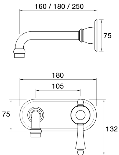
Tudor Wall Bath Mixer Set 200mm outlet incl. plate - porcelain handle A31.041.6.01 - Chrome
