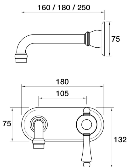
Tudor Wall Bath Mixer Set 250mm outlet incl. plate - porcelain handle A31.041.7.24 - Brushed Gunmetal
