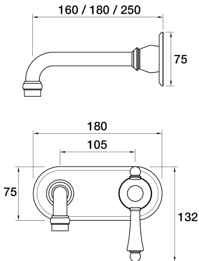
Tudor Wall Bath Mixer Set 250mm outlet incl. plate - porcelain handle A31.041.7.43 - Brass
