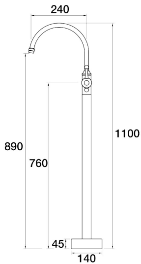
Tudor Floor Bath Filler Mixer - Gooseneck A31.072.1.21 - Brushed Rose Gold
