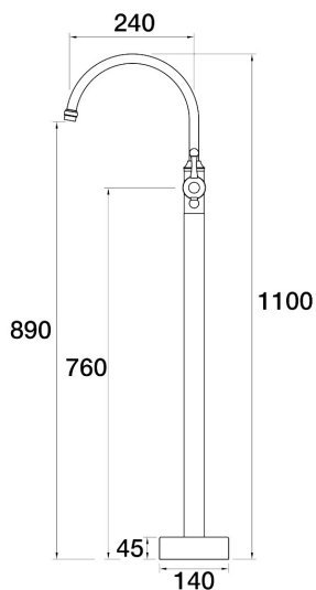
Tudor Floor Bath Filler Mixer - Gooseneck A31.072.1.39 - Antique Bronze
