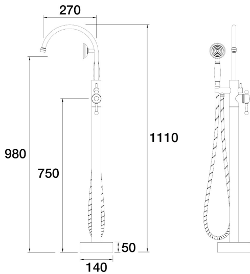
Tudor Floor Bath Filler Mixer with Handshower Gooseneck A31.075.1.01 - Chrome
