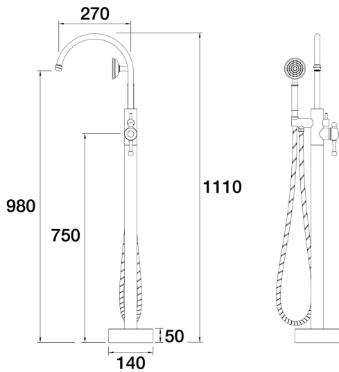
Tudor Floor Bath Filler Mixer with Handshower Gooseneck A31.075.1.23 - Gunmetal
