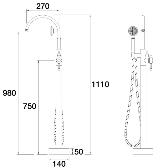
Tudor Floor Bath Filler Mixer with Handshower Gooseneck A31.075.1.54 - Volcanic Grey
