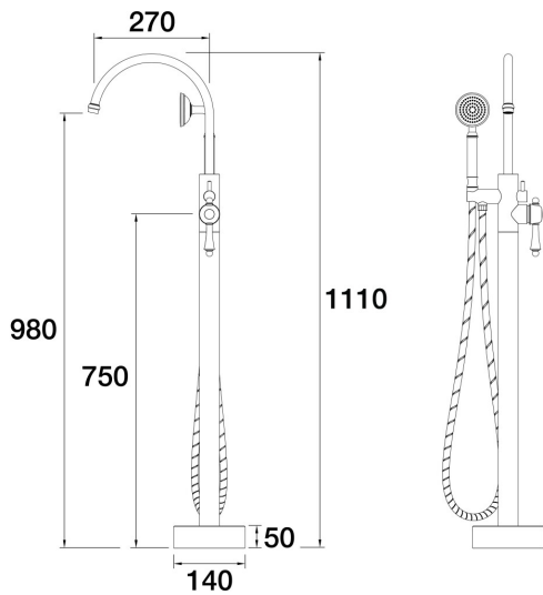
Tudor Floor Bath Filler Mixer with Handshower Porcelain Handle A31.075.2.39 - Antique Bronze
