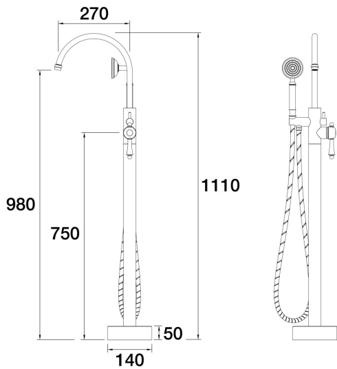
Tudor Floor Bath Filler Mixer with Handshower Porcelain Handle A31.075.2.45 - Native Brass
