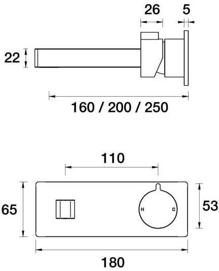
Flyte Wall Mixer on Plate 200mm A34.132.1.01 - Chrome
