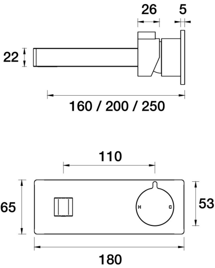
Flyte Wall Bath Mixer Set On Plate 160mm A34.141.1.01 - Chrome
