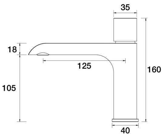
Sol Hob Basin Mixer A35.011.1.34 - Matt Black
