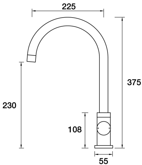
Sol Sink Gooseneck Mixer A35.026.1.39 - Antique Bronze
