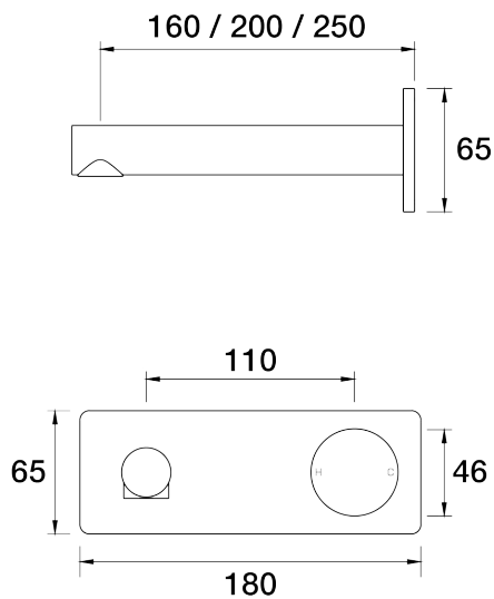
Sol Wall Mixer Basin Set 200mm outlet Incl. plate A35.032.1.01 - Chrome
