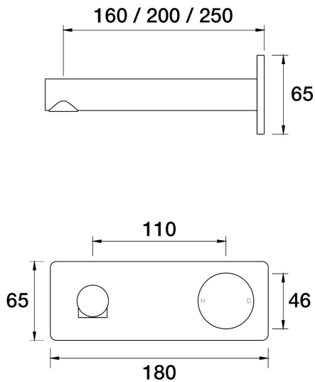
Sol Wall Mixer Basin Set 200mm outlet Incl. plate A35.032.1.27 - Satin Pearl
