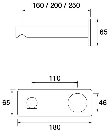
Sol Wall Mixer Basin Set 200mm outlet Incl. plate A35.032.1.39 - Antique Bronze
