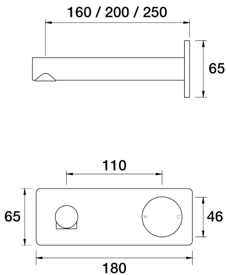
Sol Wall Mixer Basin Set 200mm outlet Incl. plate A35.032.1.48 - Copper
