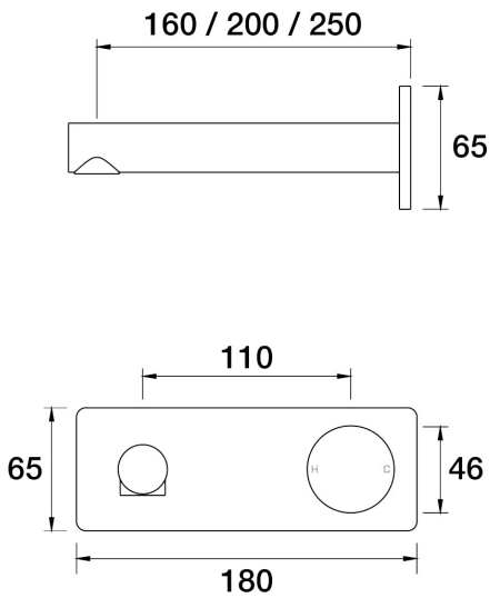
Sol Wall Mixer Basin Set 200mm outlet Incl. plate A35.032.1.70 - Sea Spray
