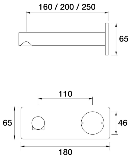
Sol Wall Mixer Basin Set 250mm outlet Incl. plate A35.032.3.45 - Native Brass
