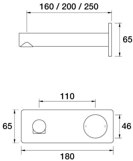
Sol Wall Bath Mixer Set 160mm outlet Incl. plate A35.041.1.57 - Matt Nickel
