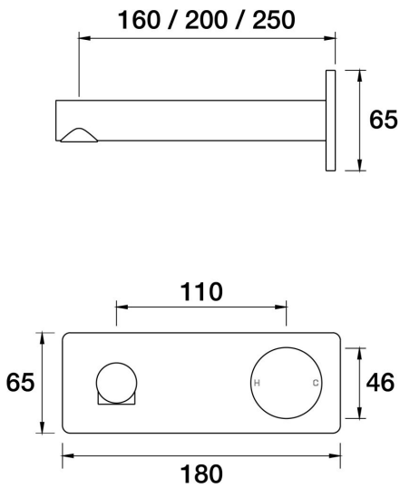
Sol Wall Bath Mixer Set 200mm outlet Incl. plate A35.041.3.01 - Chrome
