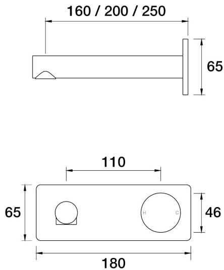
Sol Wall Bath Mixer Set 250mm outlet Incl. plate A35.041.4.44 - Antique Copper
