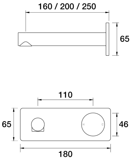
Sol Wall Bath Mixer Set 250mm outlet Incl. plate A35.041.4.75 - Forest Mist
