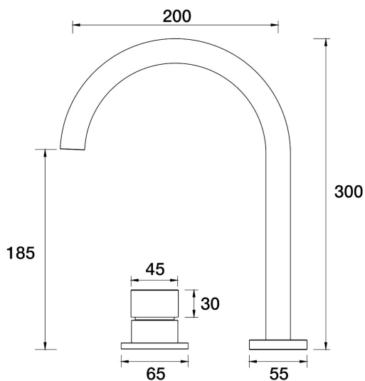
Sol Hob Mixer Set A35.081.2.48 - Copper
