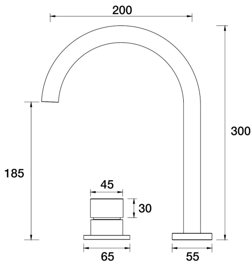
Sol Hob Mixer Set A35.081.2.78 - Umber Earth
