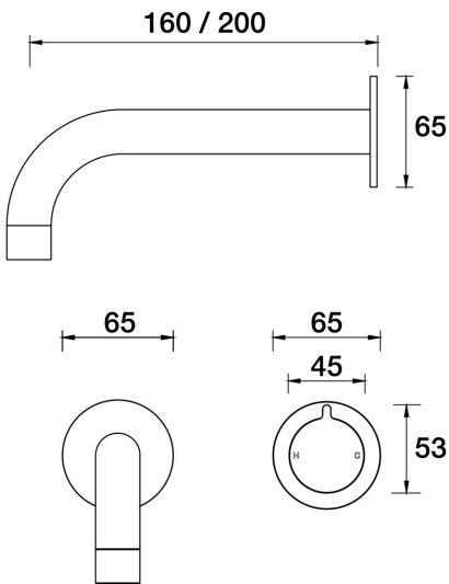
Q Wall Mixer Basin on Plate 200mm A36.032.1.34 - Matt Black
