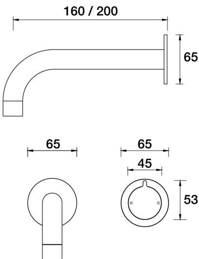
Q Wall Mixer Basin on Plate 200mm A36.032.1.42 - Brushed Copper
