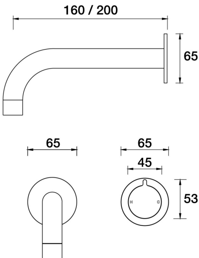
Q Wall Mixer Basin on Plate 200mm A36.032.1.47 - Luminick
