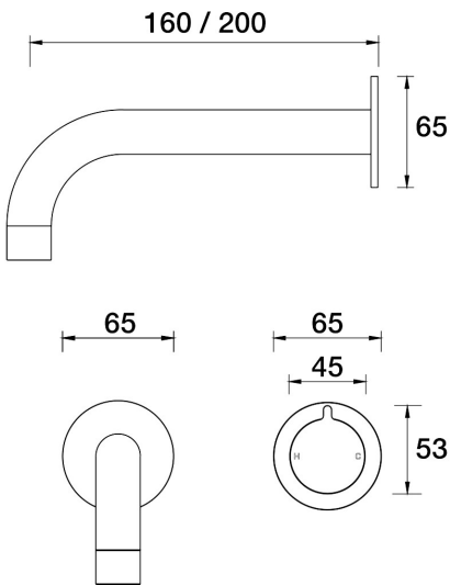
Q Wall Mixer Basin Set 200mm A36.033.1.43 - Brass
