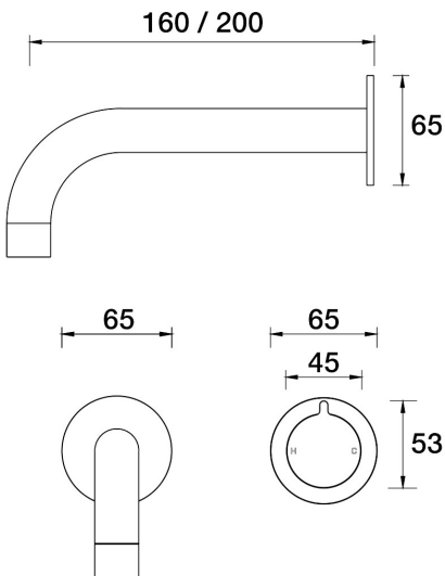
Q Wall Mixer Basin Set 200mm A36.033.1.47 - Luminick
