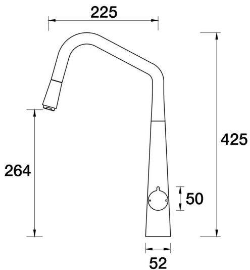
Q Sink Pull-Out Mixer A36.124.1.01 - Chrome
