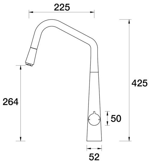
Q Sink Pull-Out Mixer A36.124.1.23 - Gunmetal
