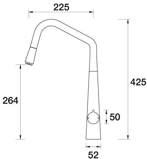
Q Sink Pull-Out Mixer A36.124.1.41 - Brushed Brass
