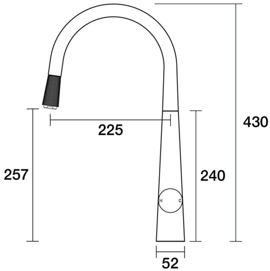
IDK Sink Pull-Out Mixer A38.024.1.01 - Chrome
