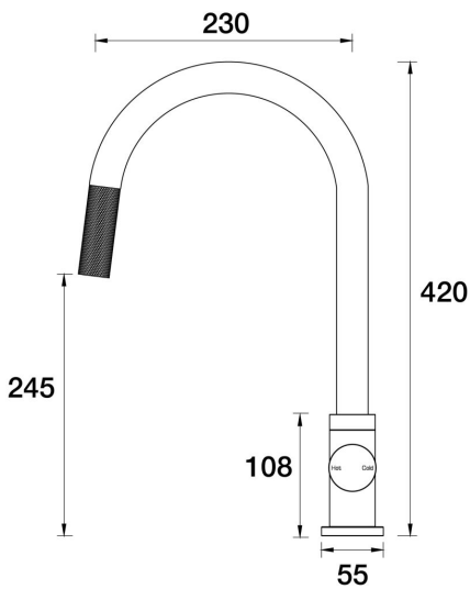
IDK Sink Pull-Out Mixer Gooseneck A38.024.2.01 - Chrome
