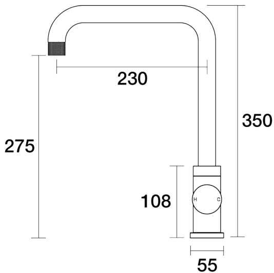
IDK Sink 90 Degree Mixer A38.025.1.01 - Chrome
