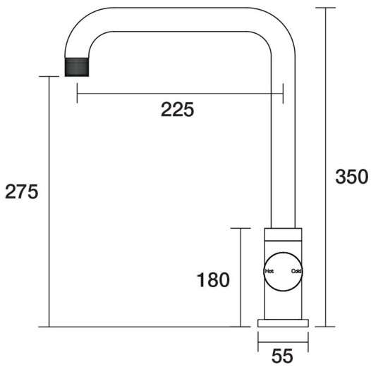
IDK Sink 90 Degree Mixer A38.025.1.01 - Chrome
