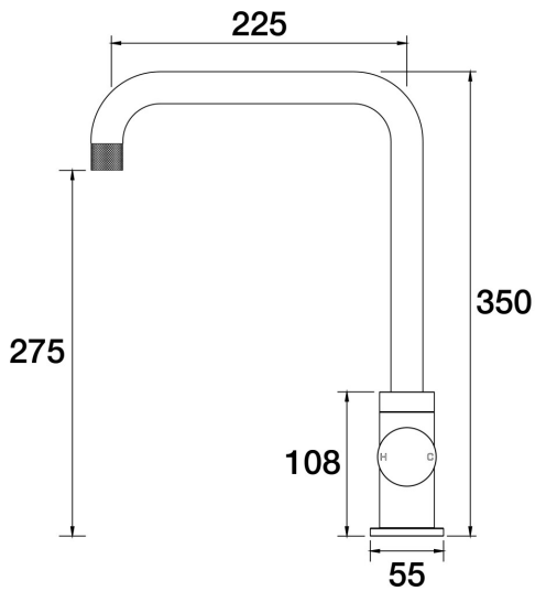
IDK Sink 90 Degree Mixer A38.025.1.32 - Midnight Black
