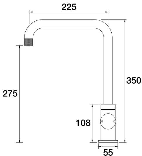
IDK Sink 90 Degree Mixer A38.025.1.57 - Matt Nickel
