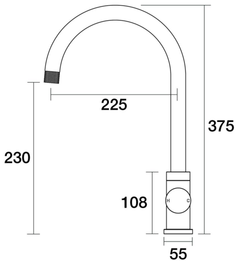
IDK Sink Gooseneck Mixer A38.026.1.01 - Chrome
