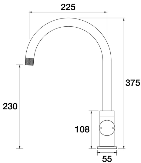
IDK Sink Gooseneck Mixer A38.026.1.25 - Brushed Nickel
