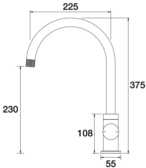
IDK Sink Gooseneck Mixer A38.026.1.45 - Native Brass
