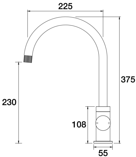
IDK Sink Gooseneck Mixer A38.026.1.52 - Burnished
