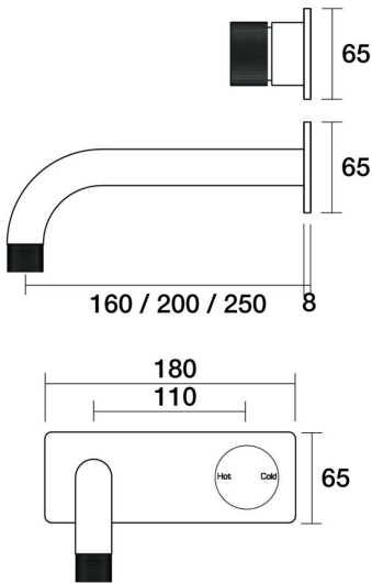
IDK Wall Mixer Basin Set 160mm outlet Incl. plate A38.032.2.01 - Chrome
