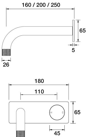
IDK Wall Mixer Basin Set 160mm outlet Incl. plate A38.032.2.25 - Brushed Nickel
