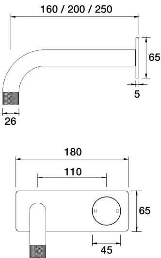
IDK Wall Mixer Basin Set 250mm outlet Incl. plate A38.032.3.39 - Antique Bronze
