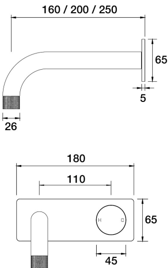
IDK Wall Mixer Basin Set 250mm outlet Incl. plate A38.032.3.57 - Matt Nickel
